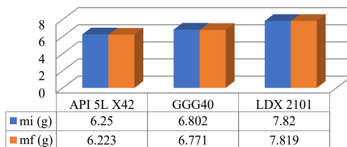
Figure 2. Weight loss of carbon steel, cast iron, and duplex stainless steel after immersion in 3 wt.% NaCl for a period of 10 days
